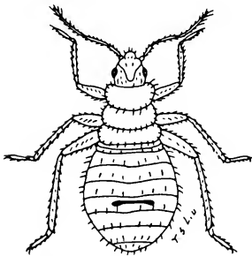
Fig. 364. Bed bug Cimex lectularius L., newly hatched.
